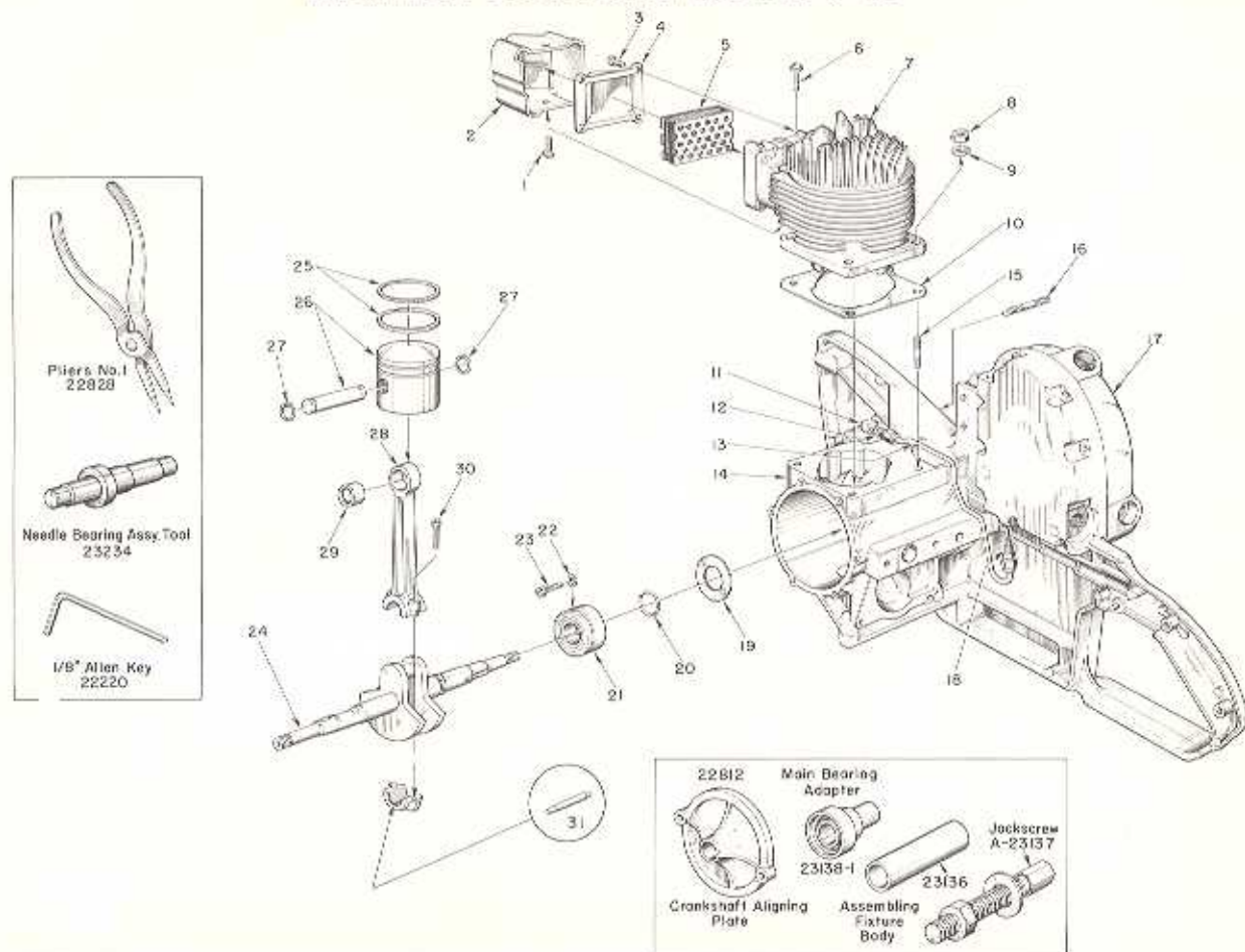
FIGURE 8 — ENGINE ASSEMBLY
