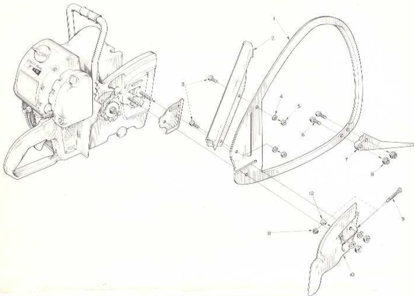
FIGURE 9 — BOW SAW PARTS
