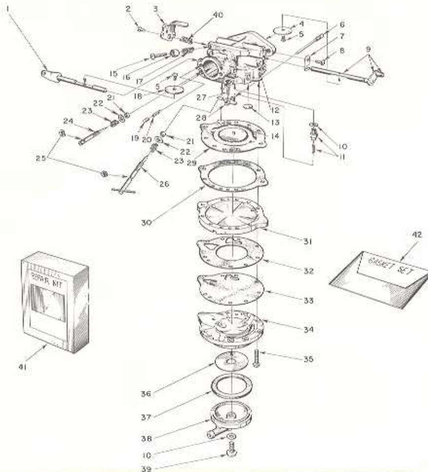
FIGURE 3 — BROWN 5-CS CARBURETOR PARTS
