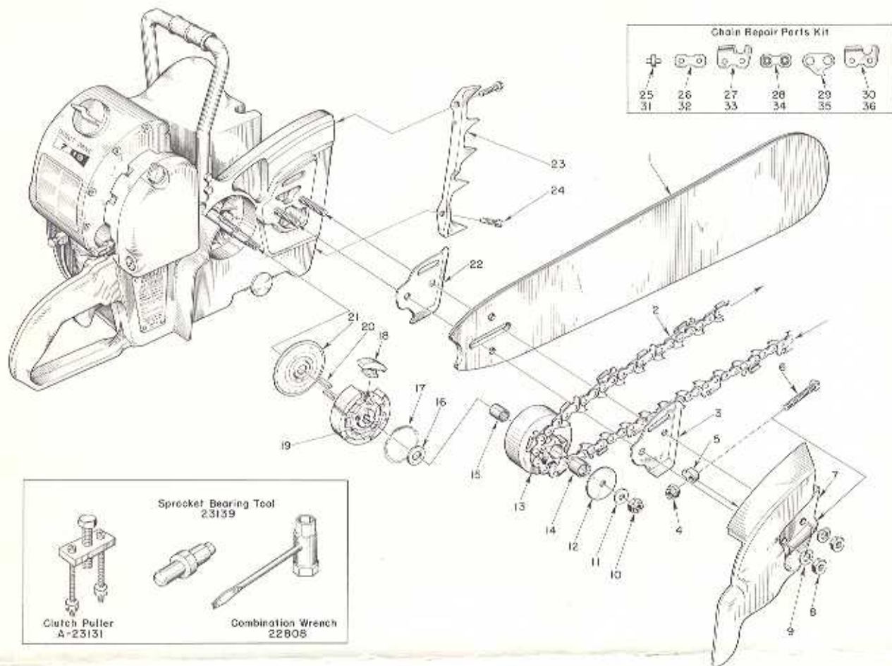
FIGURE 1 — SAW PARTS
